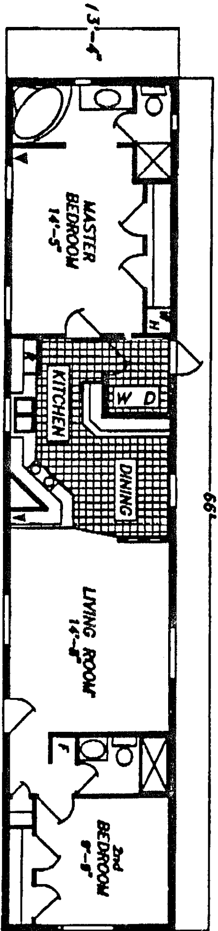
2-BEDROOM MODEL 859T 14'X70' 880 SQ.FT.
